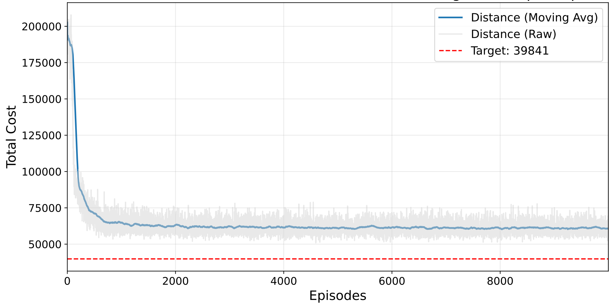
Final HYPERBAND GP Masked AutoRL-SOP Training - kro124p.2.sop
